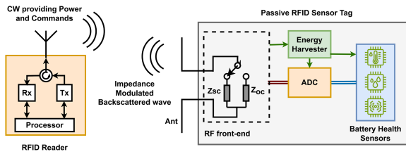
FIGURE 8. Passive RFID radio backscattering communication.
