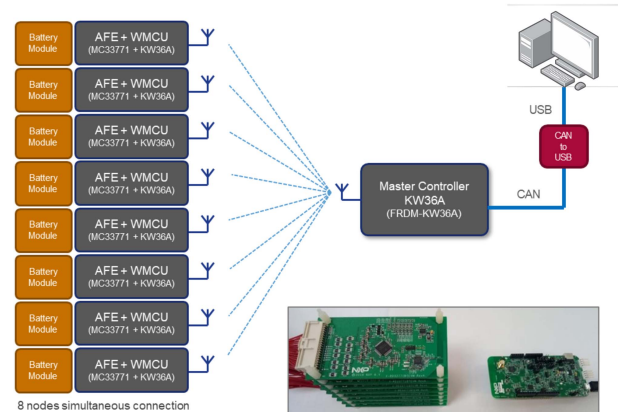
FIGURE 7. NXP Semiconductors wBMS demonstration.
