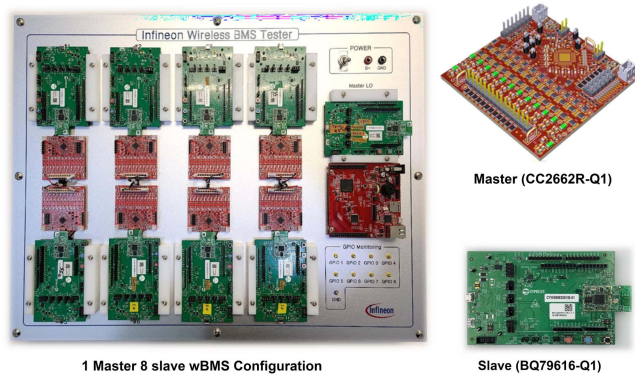
FIGURE 6. Infineon Technologies wBMS demonstration.
