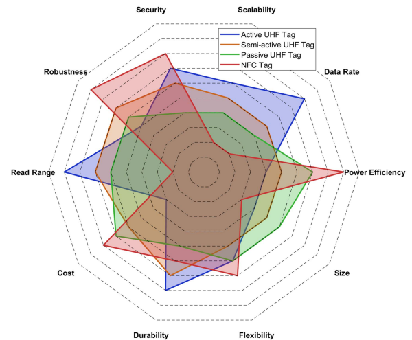
FIGURE 9. Sensing tradeoffs for RFID based active/passive tag sensors.
