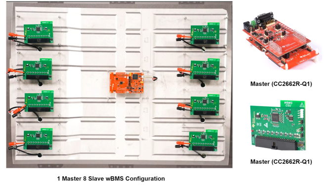
FIGURE 5. Texas Instruments wBMS demonstration.
